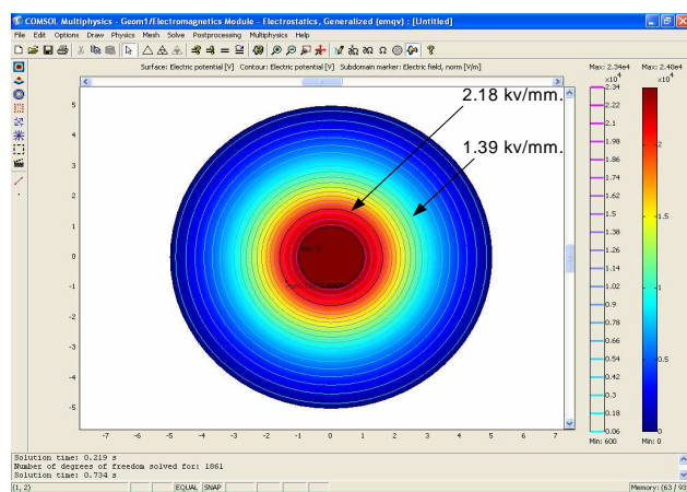
Figure 4: Show Simulations Electric Field Analysis
